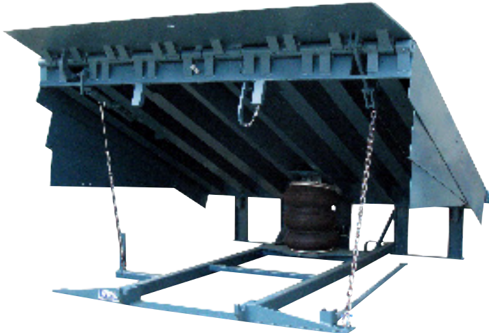
CentraAir® Series, 6' x 8', 45,000 CIR, Shown patent pending
